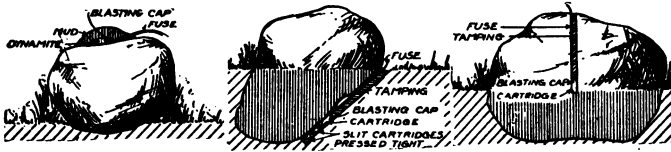
Fig. 146. Mudcapping.
